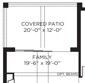
OPT. 15' SLIDER AT FAMILY ROOM
