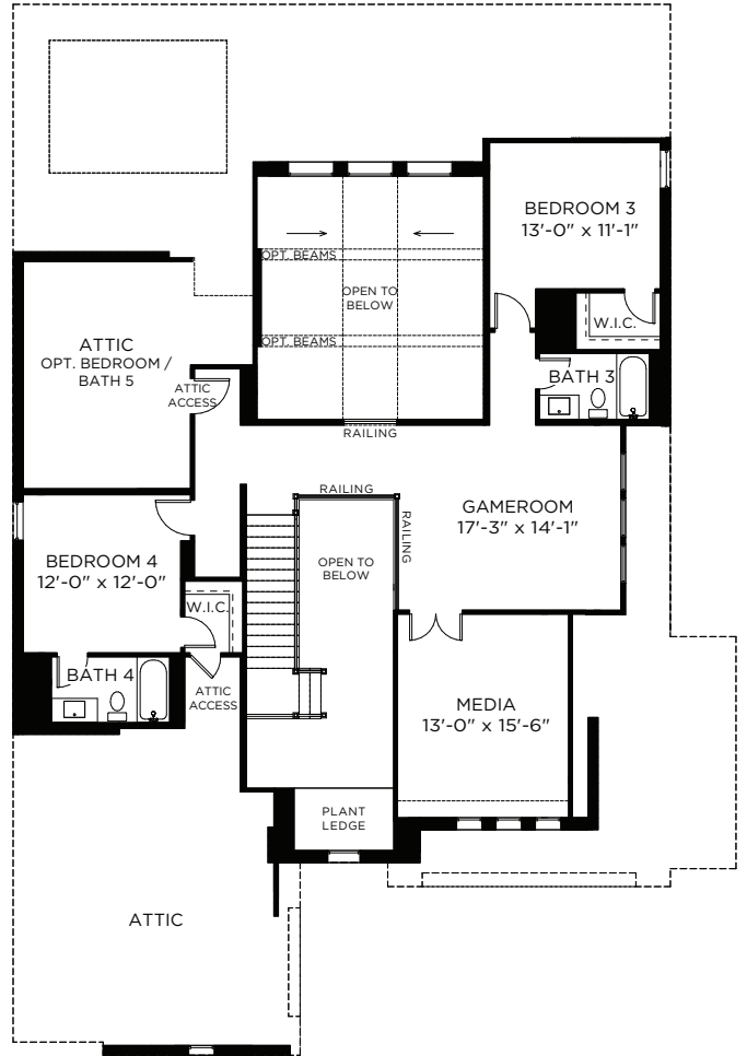
2ND FLOOR - ELEVATION A*
