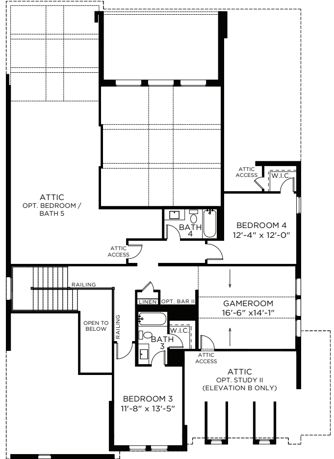
2ND FLOOR - ELEVATION A*
