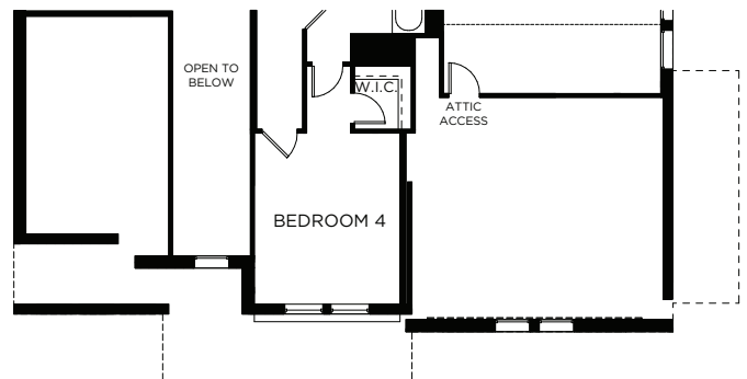
2ND FLOOR - ELEVATION B
