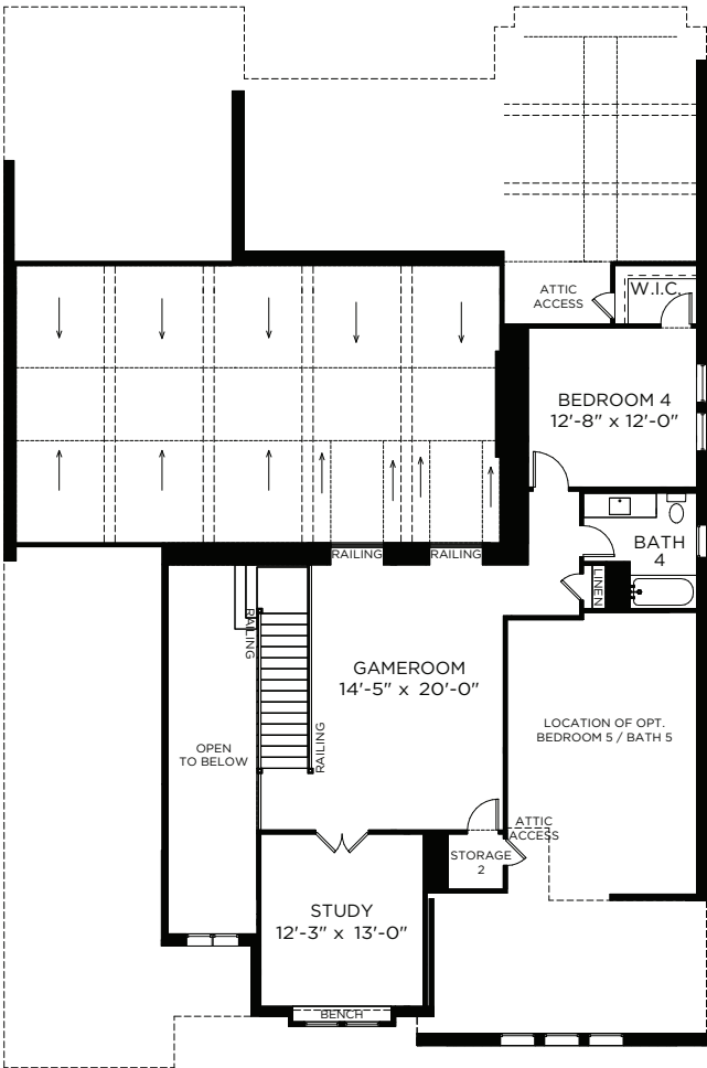
2ND FLOOR - ELEVATION A*
