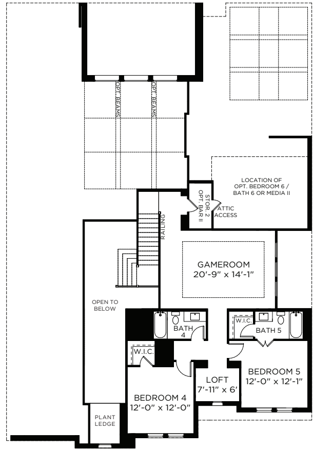
2ND FLOOR PLAN - ELEVATION A*
