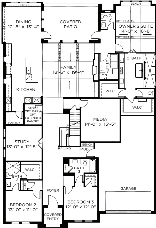
1ST FLOOR PLAN - ELEVATION A*
